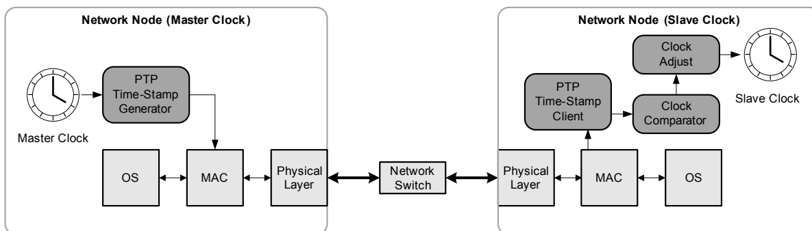
Figure 2-2. Simplified representation of synchronizing clocks using PTP
